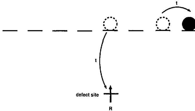
Figure 2. A defect site coupled to a uniform Bose system.
