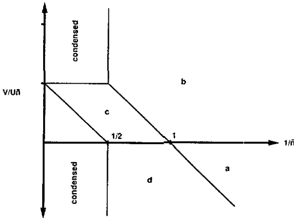
Figure 1. Trapping at weak-hopping limit. Regions (a) and (c): hole on defect. Regions (b) and (d): hole away from defect. Only regions (a) and (b) remain for non-zero hopping.
